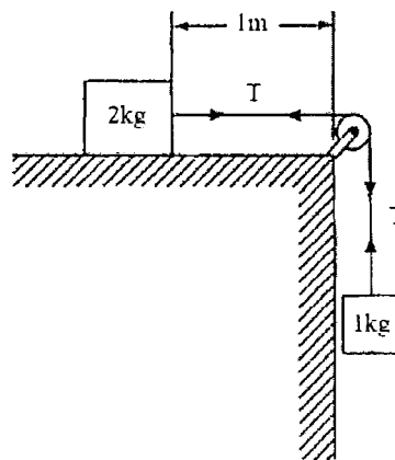
Hanging-mass system
